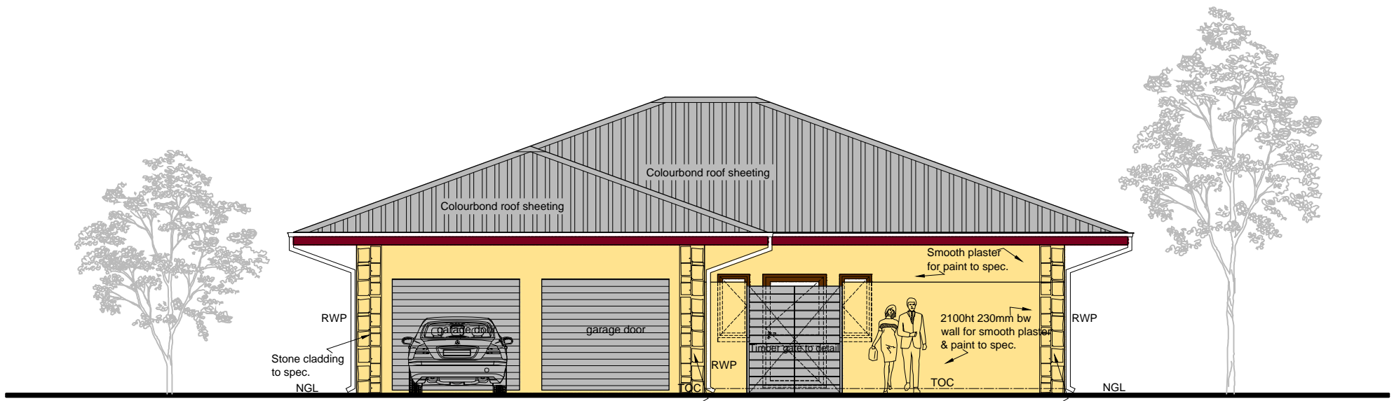
ELEVATION 1-1
